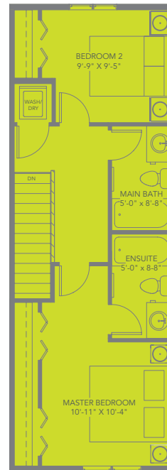
UPPER FLOOR PLAN 2 BEDROOM APPROX. 546 SQ.FT.
