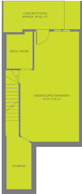
UNDEVELOPED WALKOUT BASEMENT APPROX. 384 SQ.FT. OPTIONAL DEV.
